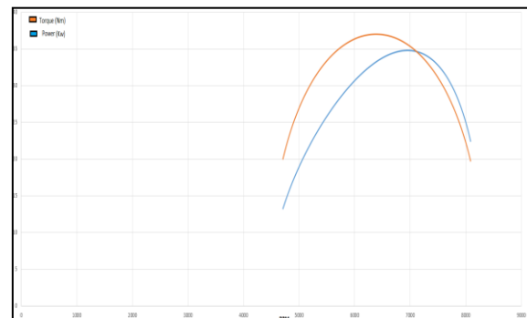
Fig 8: Obtained Power and Torque Curve
